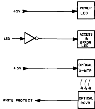
Fig. 7-22. Block diagram of optics circuit, Model 1540.
